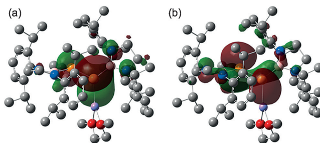
Figure 3. a) HOMO and b) HOMO-1 of 8 (dme) (only one of the two energetically similar structures is shown; hydrogen atoms omitted for clarity; color code: gray = carbon, blue = nitrogen, orange = phosphorus, pale pink = boron, purple = lithium, red = oxygen).
