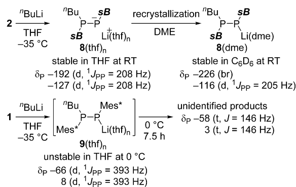
Scheme 2. Addition of n BuLi to diboryldiphosphene 1 and 2 .
