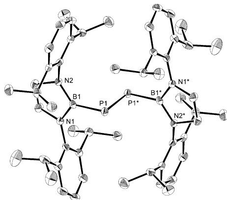
Figure 1. Molecular structure of 2 (thermal ellipsoids set at 50% probability, hydrogen atoms omitted for clarity; asterisks denote atoms generated by symmetry operation). Selected bond lengths [Å] and angles [°]: P1–B1 1.936(3), N1–B1 1.418(4), N2–B1 1.424(4), P1–P1* 2.0655(17); P1*–P1–B1 95.83(9), N1–B1–N2 108.3(2), P1–P1–B1–N1 95.8(2).
