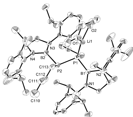
Figure 2. Molecular structure of 8 (dme) (thermal ellipsoids set at 50% probability, hydrogen atoms omitted for clarity). Selected bond lengths [Å] and angles [°]: N1–B1 1.448 (4), N2–B1 1.457 (4), P1–B1 1.896 (3); N1–B1–N2 105.2(17) N3–B2 1.445 (4), N4–B2 1.434 (4), P2–B2 1.933 (3), P1–P2 2.1775 (11).
