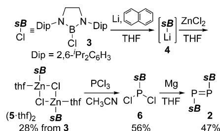
Scheme 1. Synthesis of diboryldiphosphene 2 .
